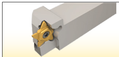
PCHR/L-24-JHP-MC tools with bottom fed high pressure coolant system
