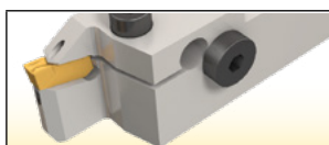
GHDR/L-JHP (short pocket) tools with high pressure coolant system
