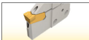
CGPAD-JHP interchangeable adapters with internal channels for high pressure coolant
