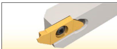
SCHR/L-22BF square shank tools with back and front clamping for swiss-type and automatic machines
