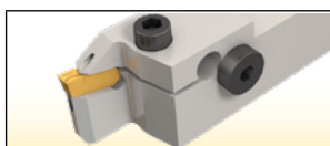
GHDR/L-JHP-MC (short pocket) tools with bottom fed high pressure coolant system
