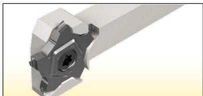
PCHR/L-24 square shank tools
