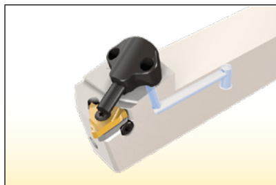
SER/L-JHP-MC tools with bottom fed high pressure Coolant System
