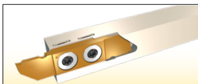
SCHR/L-41BF square shank tools with back and front clamping for swiss-type and automatic machines
