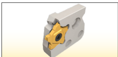
PCADR/L-JHP interchangeable adapters with internal channels for high pressure coolant
