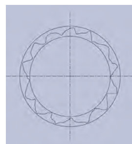
Figure 1: Typical lobed hole geometry generated by multi-fluted reamer.
