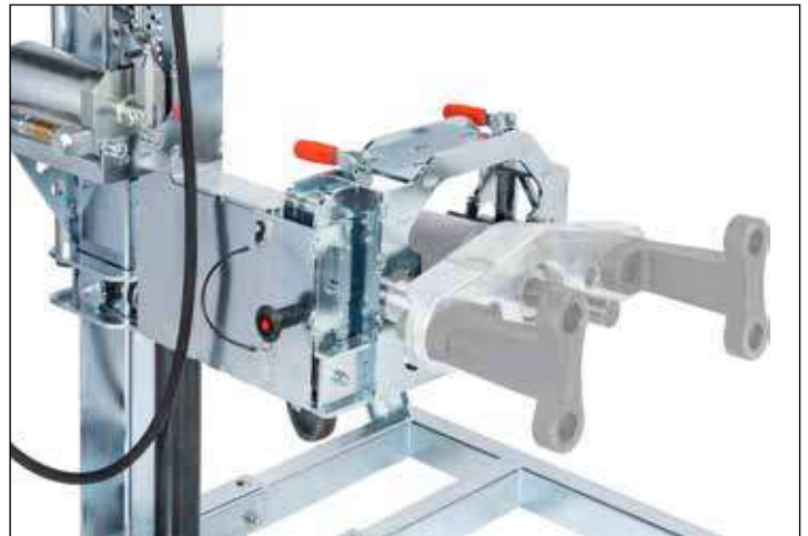
Stud bolt extension for hubs
