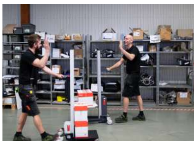
LOGISTIC
